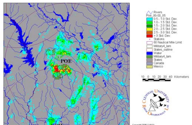
Map of important migration stopover areas for Fort Polk, LA. The colors represent standard deviations of above the mean density of birds per cubic km. Note that many of the stopover areas are associated with riparian habitat.
