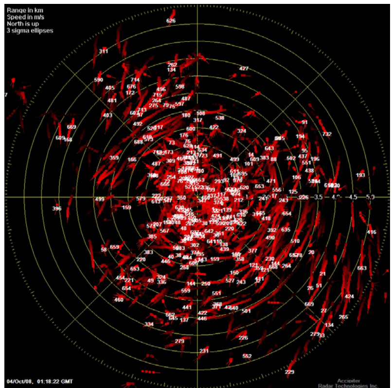
Targets being tracked by an eBirdRad digital avian radar system at Edisto Island, SC, 4 October 2008 01:18:22 UTC (21:18:22 EDT). The length of the red "tails" represents the history of a target's positions in the scans prior to this image being taken. The white numeric labels (Track IDs) show the current position of the targets being tracked by the radar (total = 234); tails with no label are targets that are no longer being tracked by the radar.
