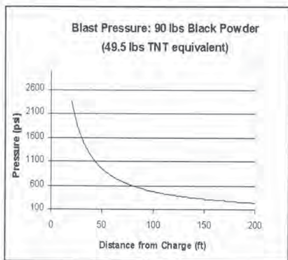
Figure 9.5. Blast pressure.
