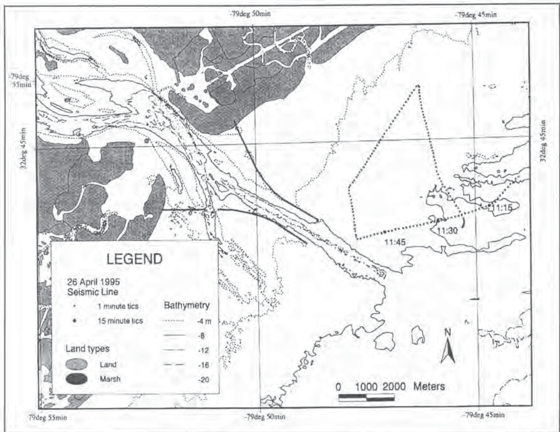
Figure 9.3. Deep penetration sub-bottom transect.
