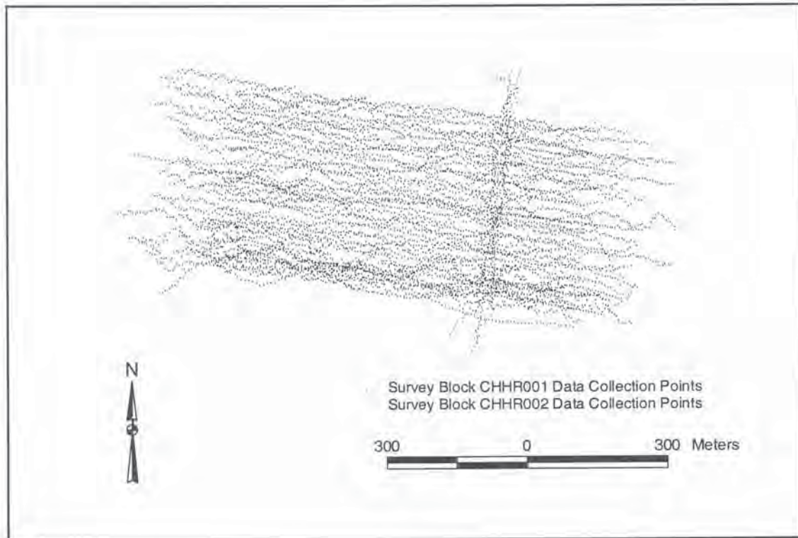
Figure 6.7. Data sample points collected during the H.L. Hunley predisturbance magnetometer survey.
