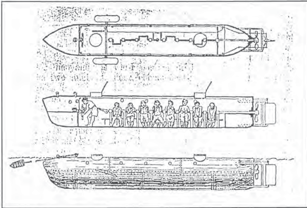
Figure 8.1. Simon Lake's 1899 drawing of Hunley . Though inaccurate in many details, it is the only historical depiction that includes deadlights.
