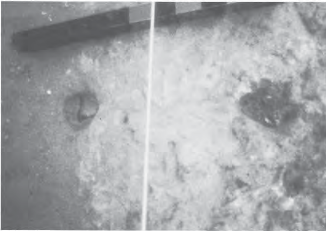
Figure 8.11. Plan view of twin deadlights on either side of vessel centerline. SCIAA photo by Christopher Amer.
