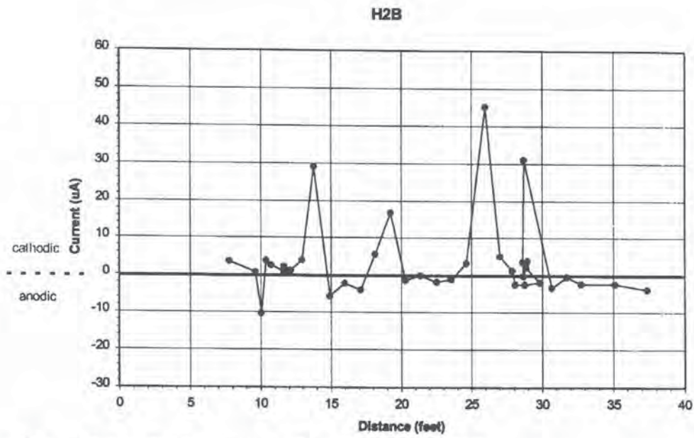
Figure 9.10. Surface current flux for transect H2B.
